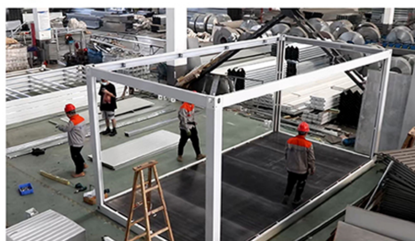
5 Install floor board with flat screws
