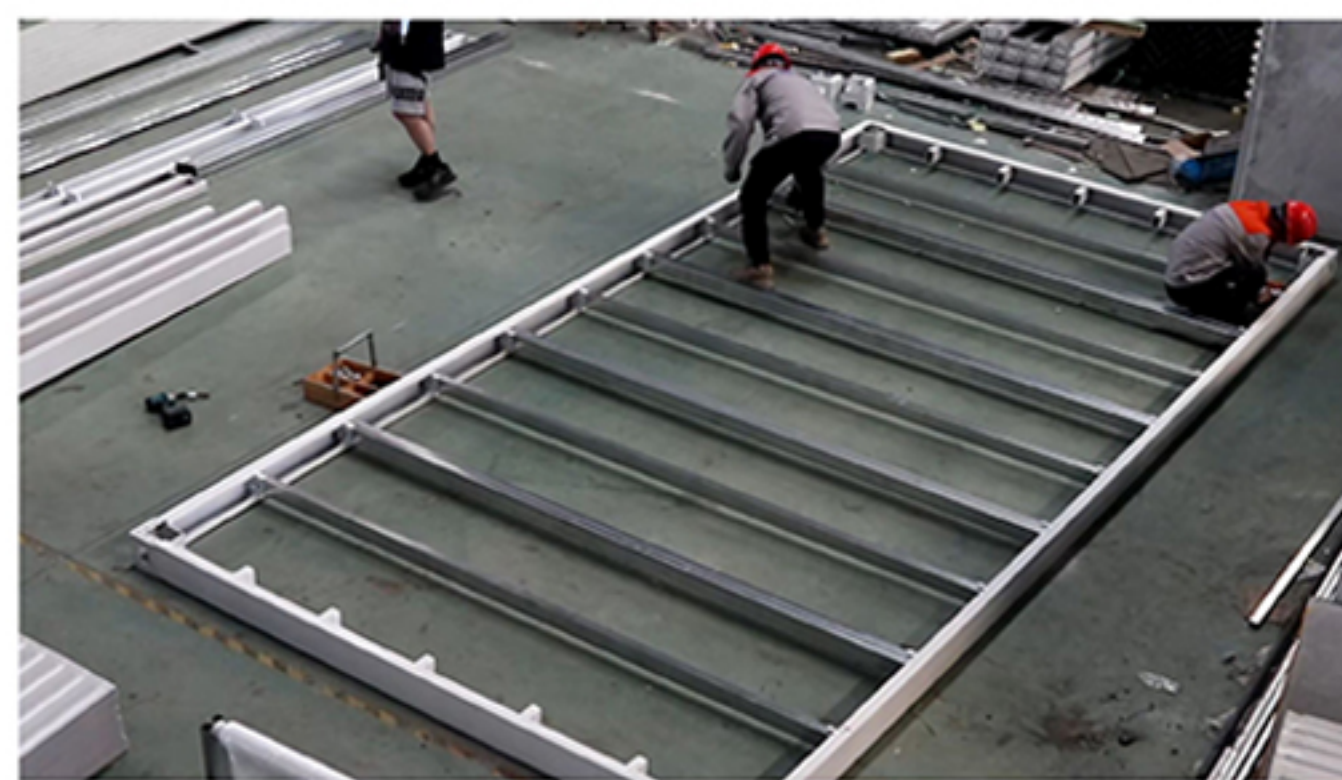
2 Install floor purlins
