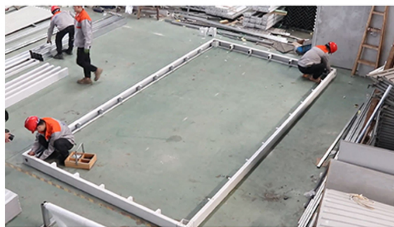
1 Put floor beam and floor fittings in order
